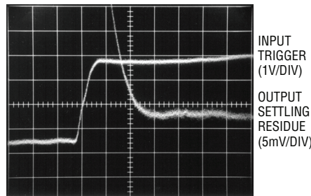
0.1% Settling Time
